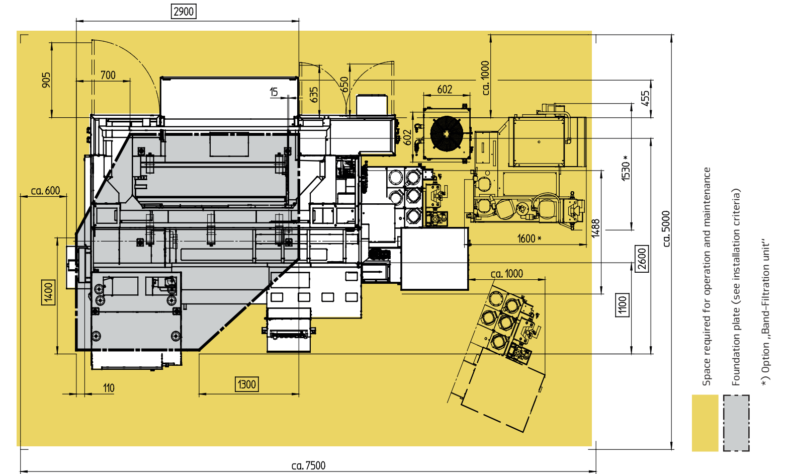
HT65 PM machine layout with paper-band filter system and chip conveyor
