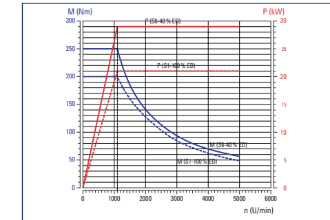
Main and counter spindle \varnothing 65 mm / \varnothing 76 mm
